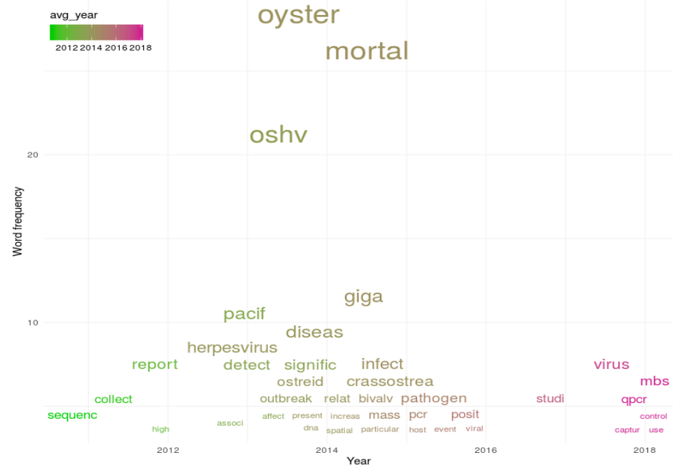
Top 30 words from articles with keywords oyster and herpesvirus word frequency (size) ~ year (color)
