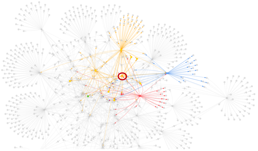
Top 30 words from articles with keywords oyster and herpesvirus word frequency (size) ~ year (color)
