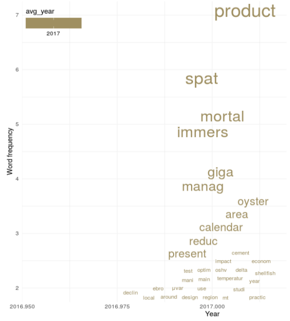
Top 30 words from articles with keywords oyster and herpesvirus word frequency (size) ~ year (color)
